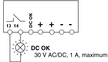
Figure 10 Floating contact
