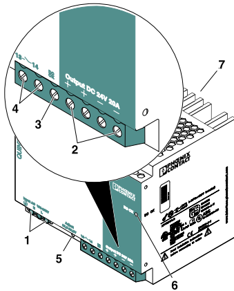
Figure 1 Operating elements
