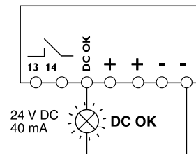
Figure 11 Active signal output
