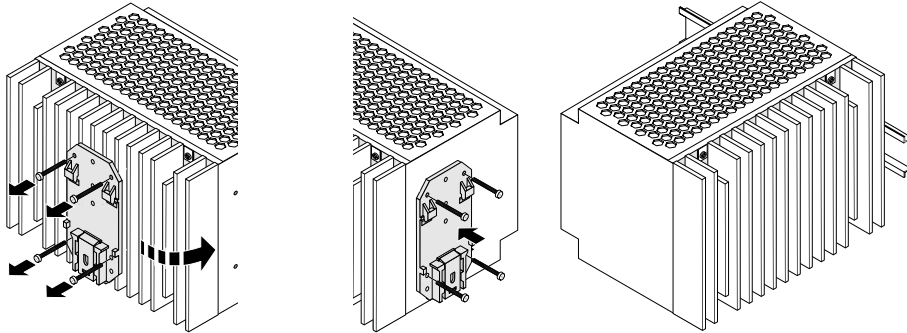
Figure 6 Narrow mounting position
