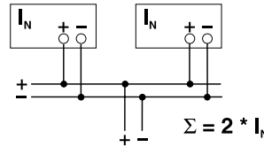
Figure 16 Increasing power
