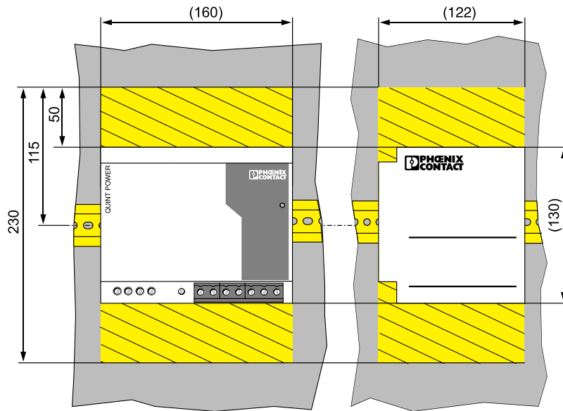
Figure 4 Mounting position (dimensions in mm)
