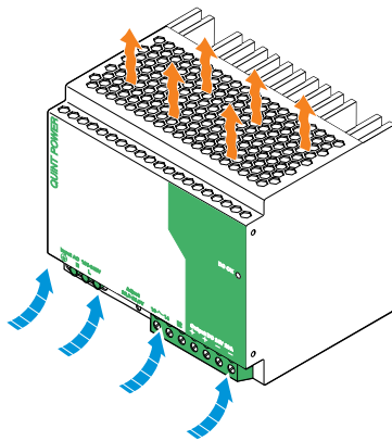
Figure 3 Convection
