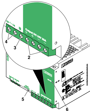
Figure 9 Output
