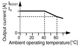
Figure 14 Temperature response
