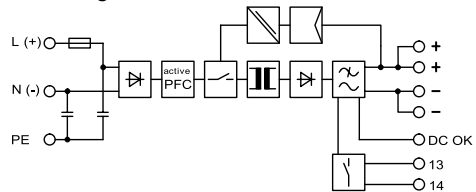
Figure 2 Block diagram
