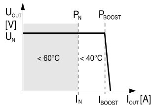
Figure 13 Output characteristic curve
