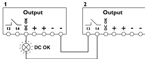
Figure 12 Signal loop
