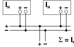
Figure 15 Redundancy operation
