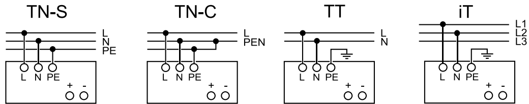
Figure 7 100...240 V AC networks
