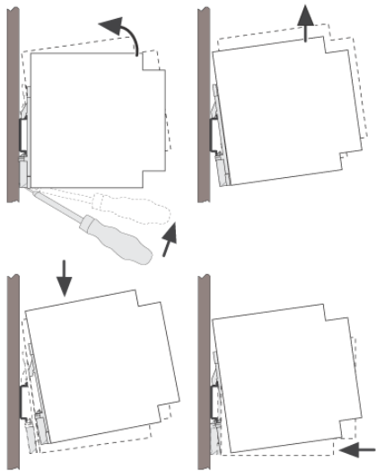
Figure 5 Flat mounting position
