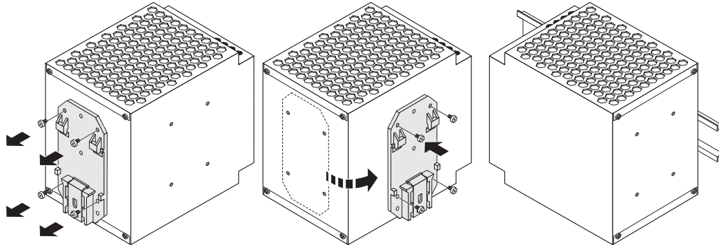
Figure 6 Flat mounting position
