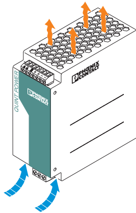
Figure 3 Convection
