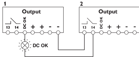
Figure 12 Signal loop
