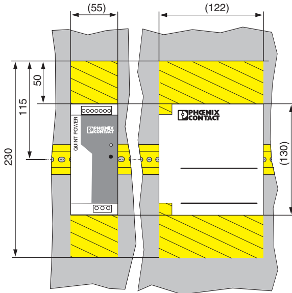
Figure 4 Mounting position (dimensions in mm)
