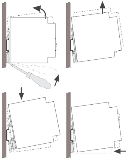
Figure 5 Narrow mounting position
