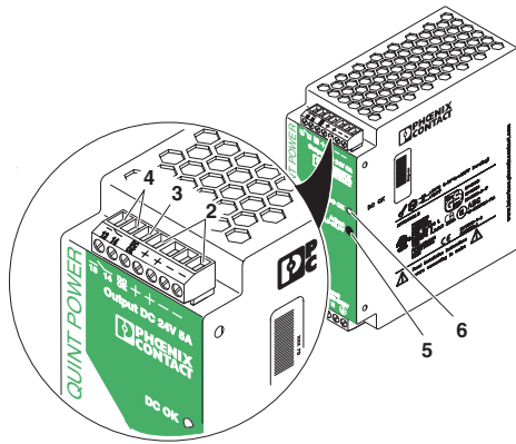
Figure 9 Output
