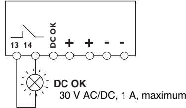
Figure 10 Floating contact
