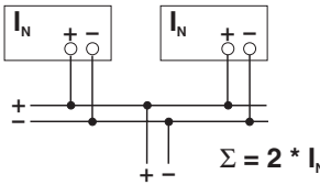
Figure 16 Increasing power
