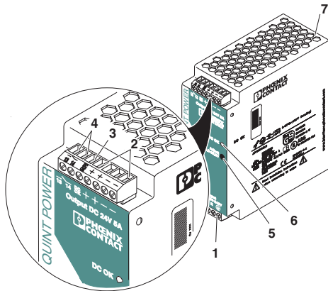
Figure 1 Operating elements
