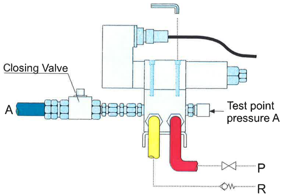
DETAILED SYMBOL
