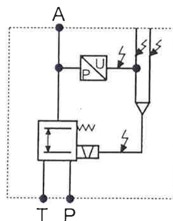
SIMPLIFIED SYMBOL
