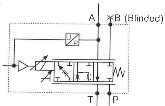
DETAILED SYMBOL
